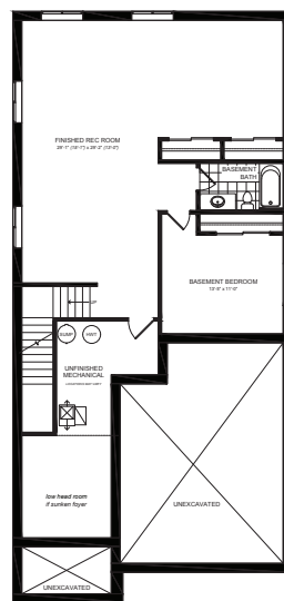
OPT. FINISHED BASEMENT 1,178 SQ.FT.
